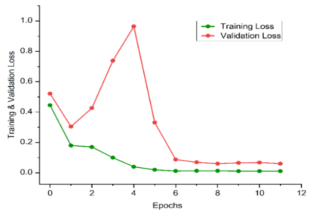
Fig. 3: Epochs vs. Training and Validation Loss
