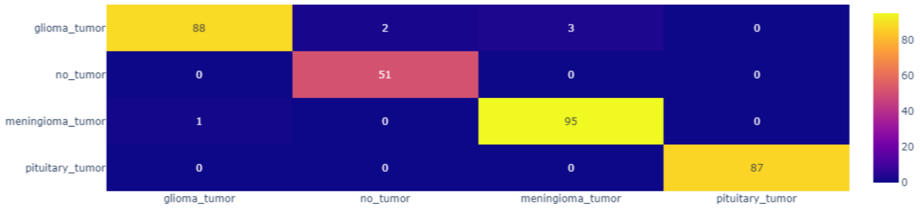
Fig. 5: Heatmap of the Confusion Matrix
